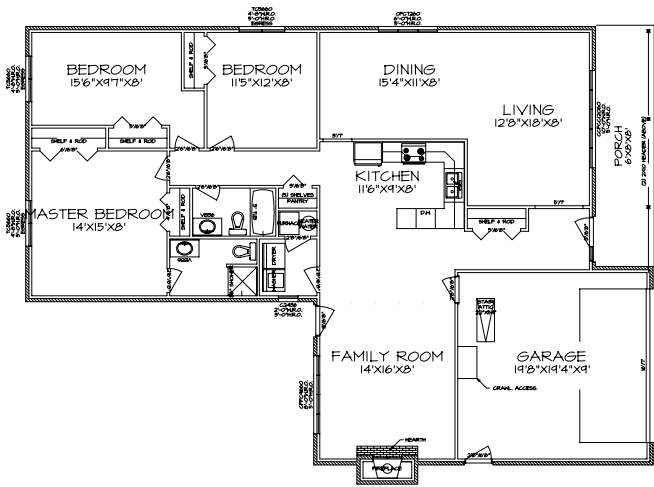
FIRST FLOOR PLAN A-4 SCALE: 1/4"=1'-0"
